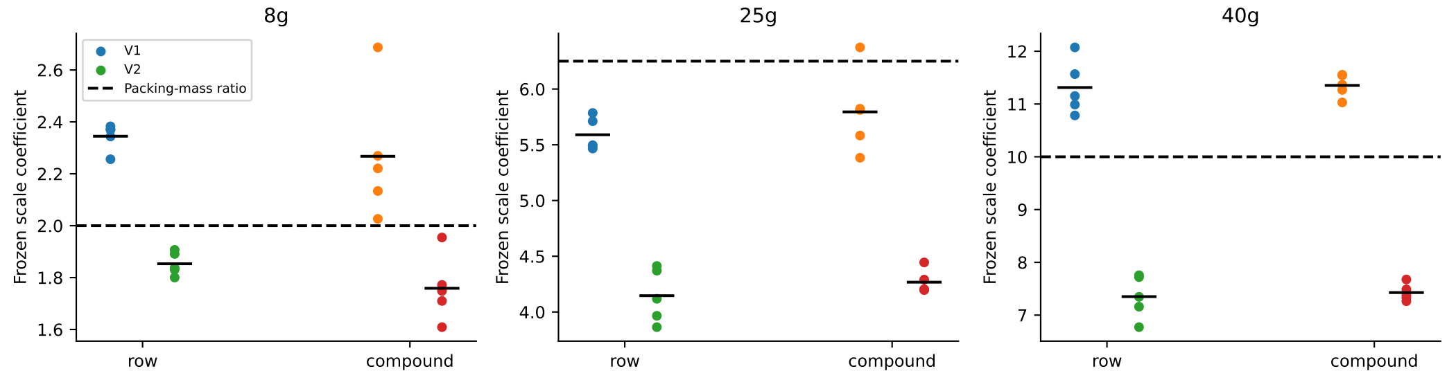
Budget 100: empirical coefficients versus nominal mass ratio
