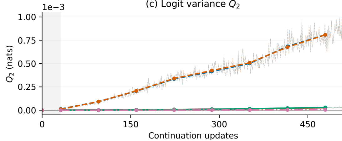
(c) Logit variance Q_2
