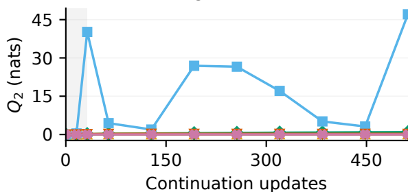
(c) Logit variance Q_2
