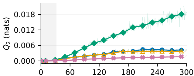
(c) Logit variance Q_2
