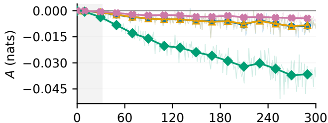
(b) Linear response A
