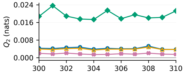
Logit variance Q_2
