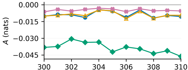
Linear response A
