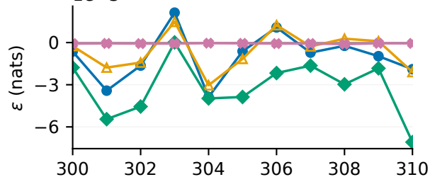
1e-3 Remaining response \varepsilon
