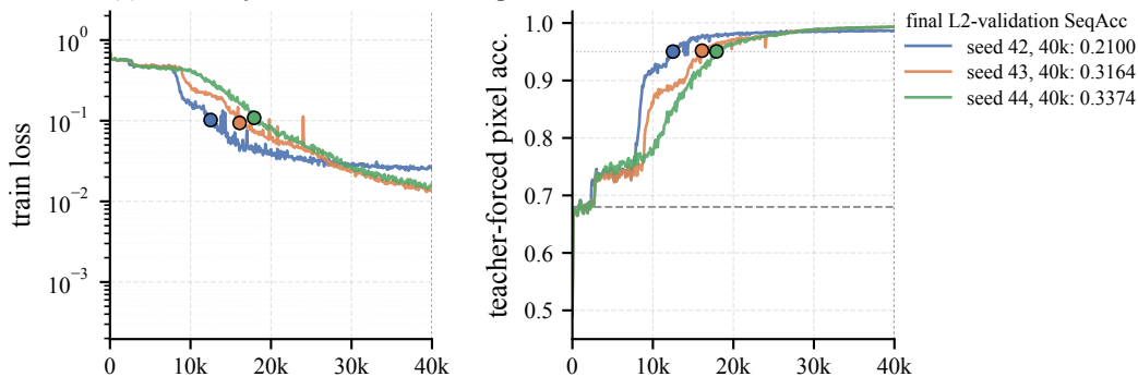
(b) d128, 4 layers, 4 heads, 924,801 parameters
