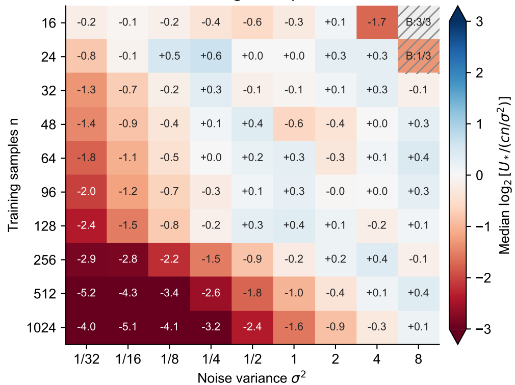
Deviation from the straight-line prediction
