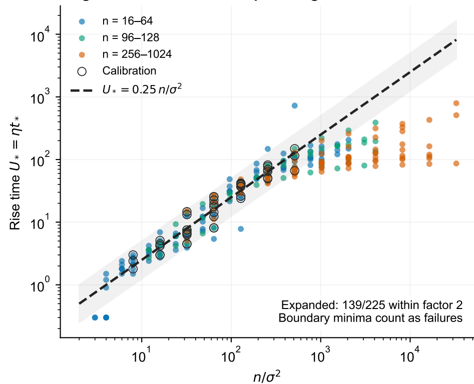
Original interaction task: expanded grid
