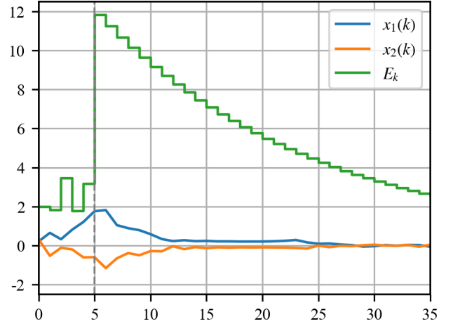
Fig. 1: State components x_1(k) (blue), x_2(k) (orange), and radius of quantization range E_k (green) over 35 simulation steps.
