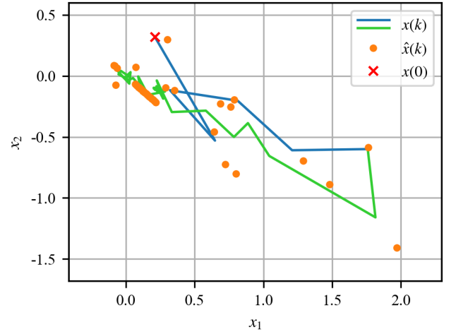
Fig. 2: State-space trajectory of x(k) (blue: controller design stage; green: feedback stabilization stage) and quantized measurements \hat{x}(k) (orange). The initial state is indicated by a cross.
