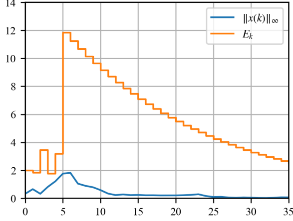
Figure 1: State norm \|x(k)\|_\infty (blue) and quantization bound E_k (orange) over 35 simulation steps. The transition from controller design stage to feedback stabilization stage occurs at step 5.
