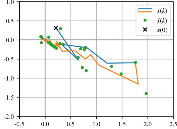
Figure 2: State-space trajectory x(k) (blue: controller design stage; orange: feedback stabilization stage) and quantized measurements \hat{x}(k) (green). The initial state is indicated by a cross.
