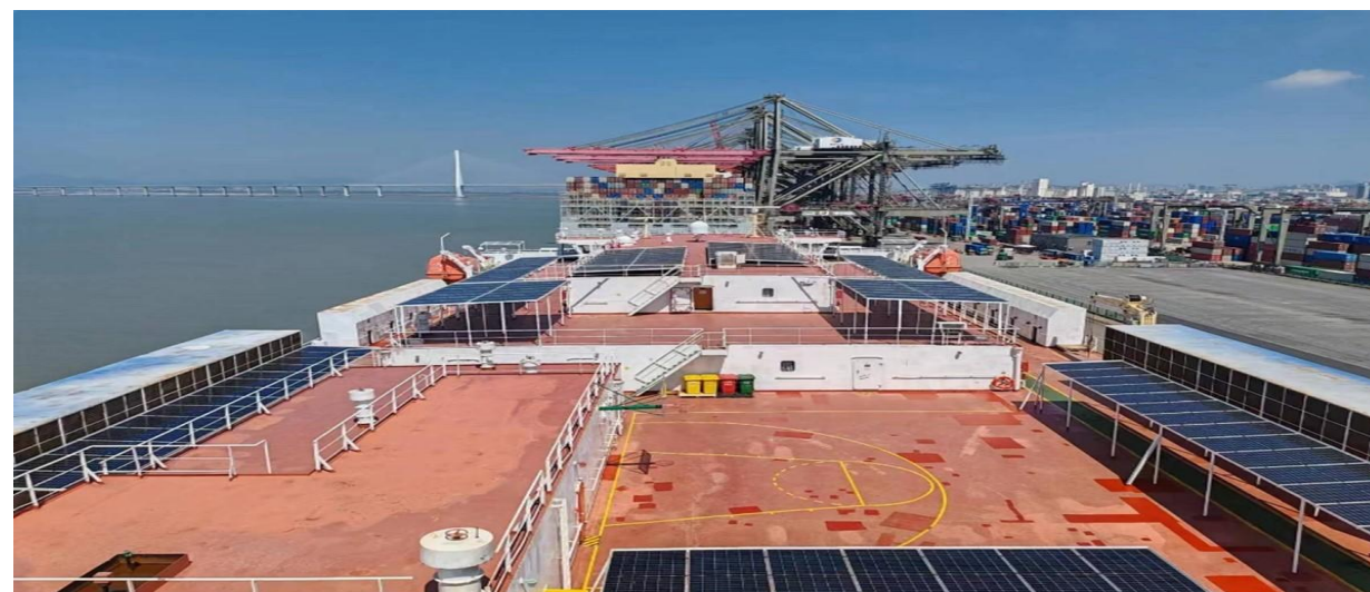
“中远盛世”轮光伏阵列布置
