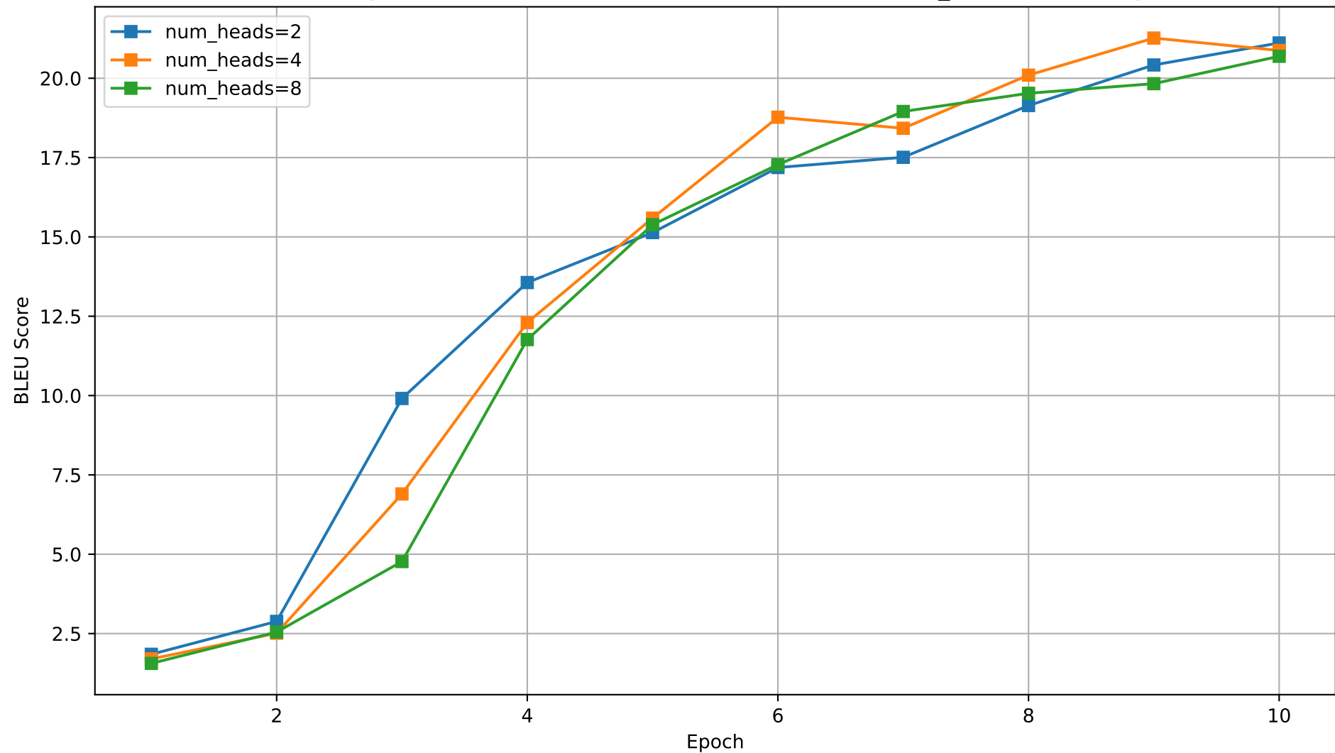
BLEU Score Comparison of Different Number of Attention Heads (d_model=384, dropout=0.1)
