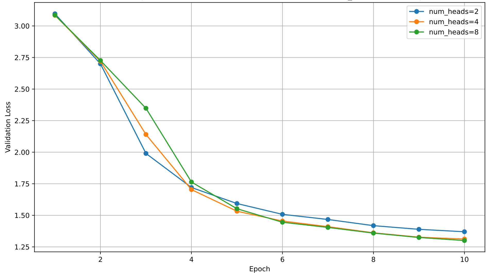
Validation Loss Comparison of Different Number of Attention Heads (d_model=384, dropout=0.1)
