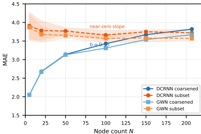
(c) Coarsened vs. subset (METR-LA)
