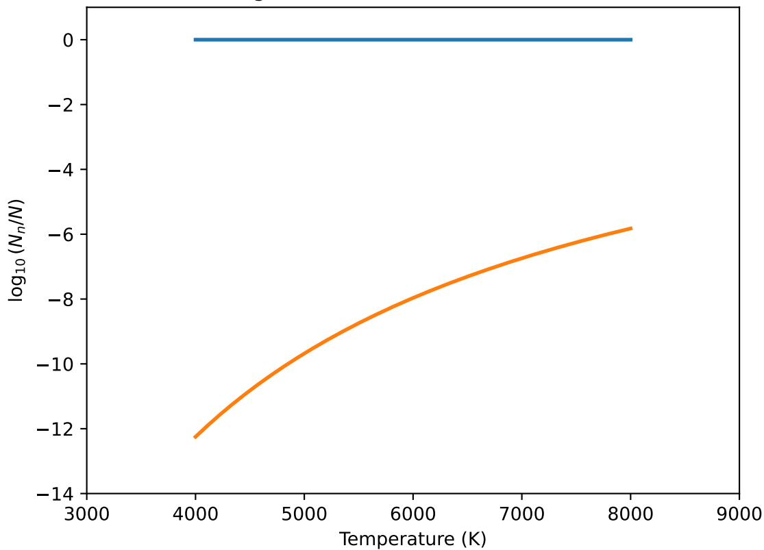
Fig 1.9-like: H excitation (n=1,2)
