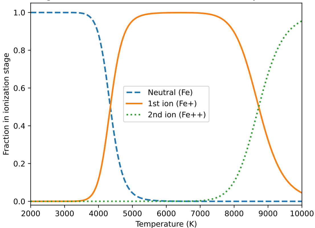
Fig 1.10-like: Iron ionization fractions ( P_e = 1 \text{ dyne/cm}^2 )
