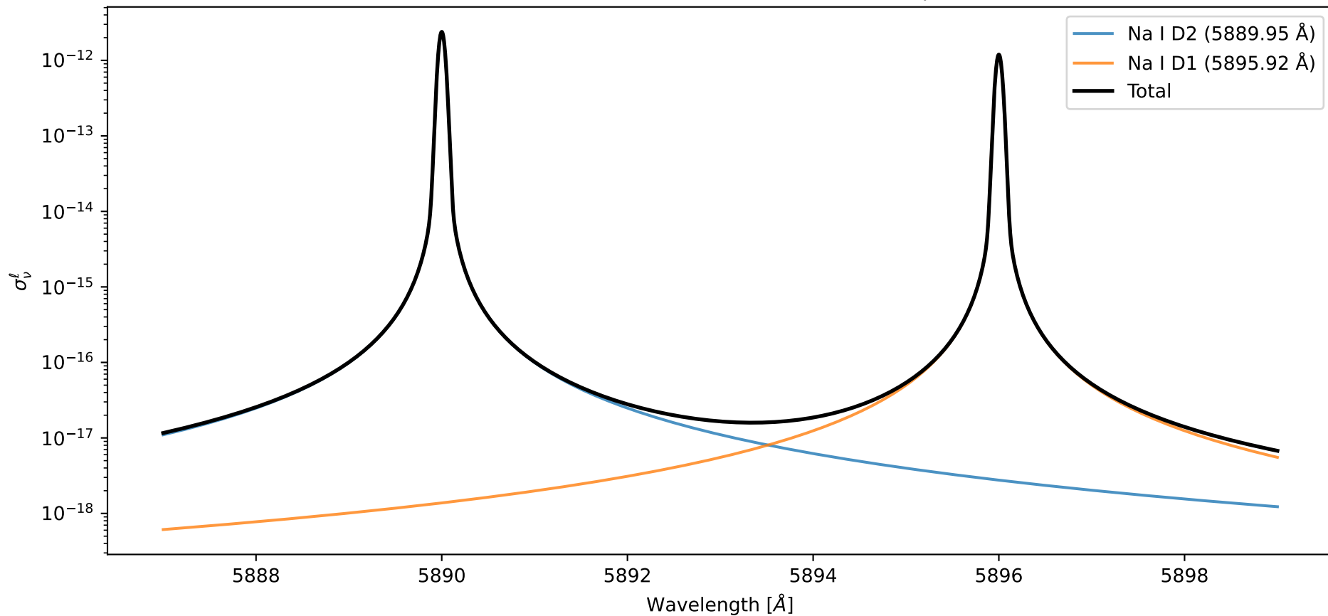
Na I D Doublet Monochromatic Line Extinction per Particle
