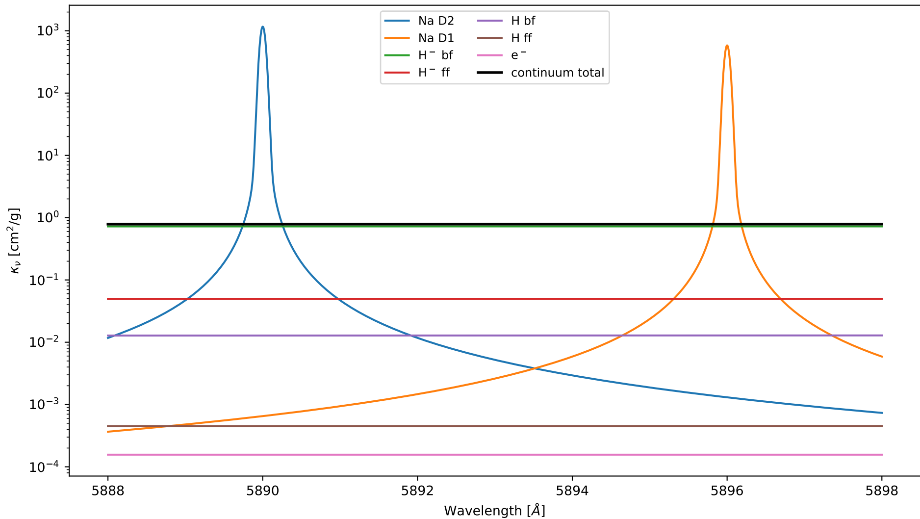
Na I D Line and Continuum Opacity at \tau_{500} \approx 1
