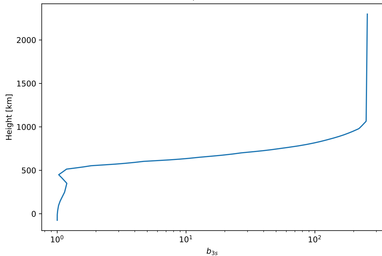
Na I 3s Departure Coefficient
