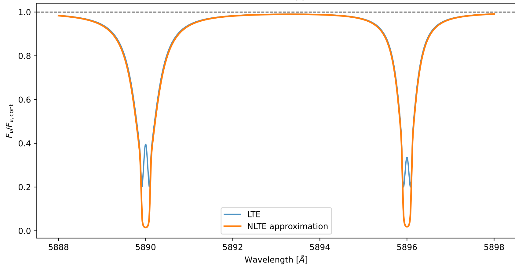
Na I D: LTE vs NLTE Approximation
