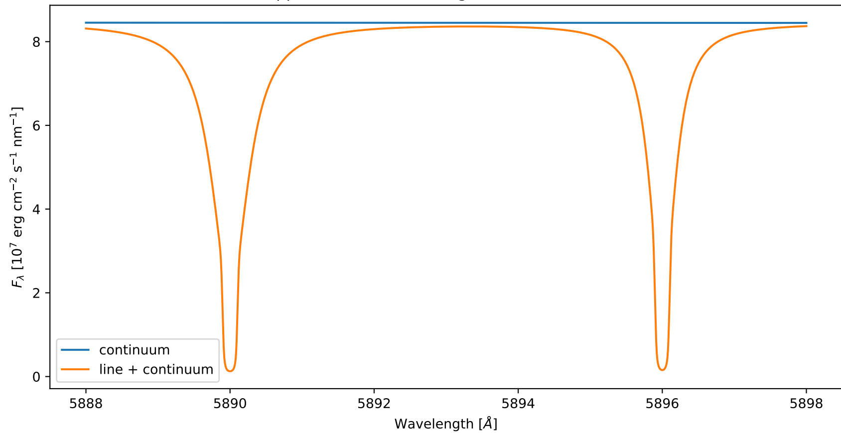
Approximate NLTE Emergent Flux near Na I D
