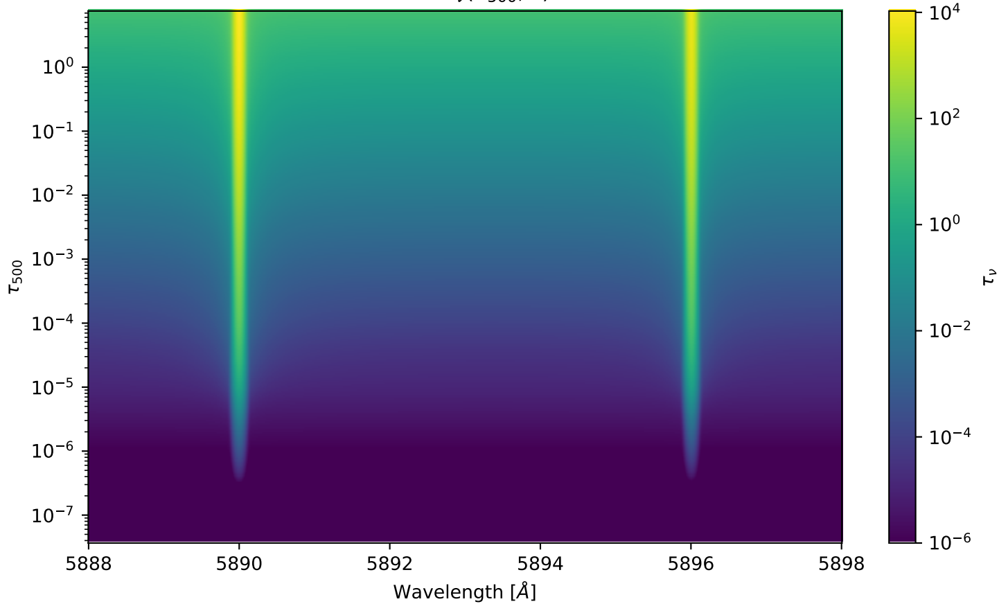
NLTE \tau_\nu(\tau_{500}, \lambda)
