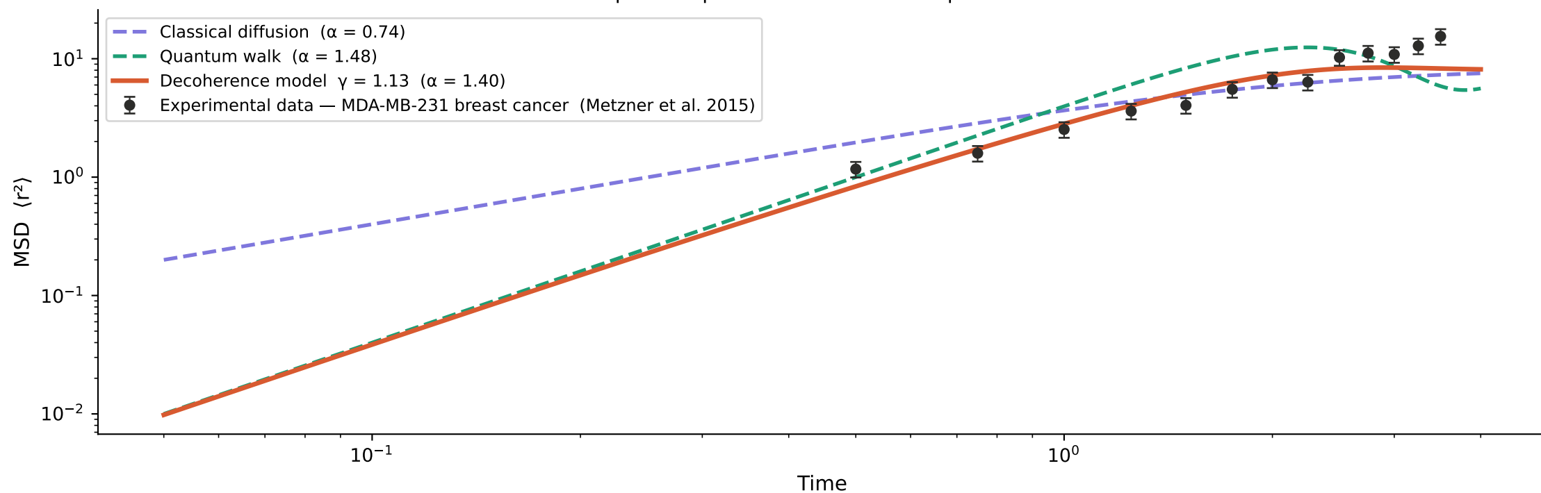
Mean-square displacement: model vs experimental data
