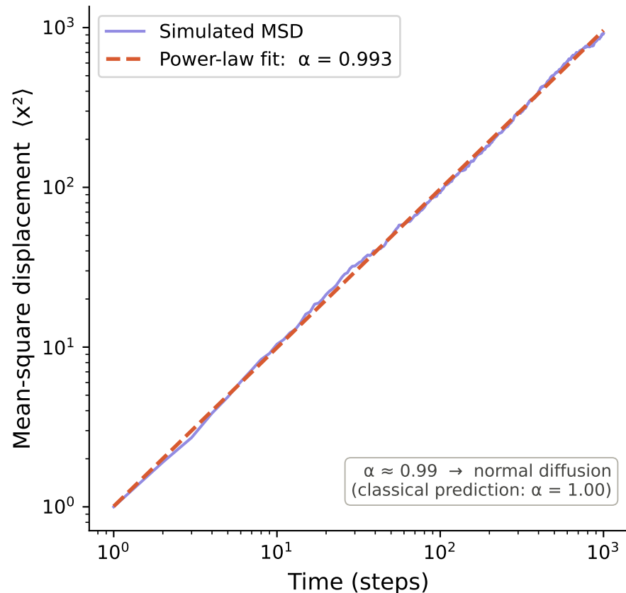
MSD vs time (log-log scale)
