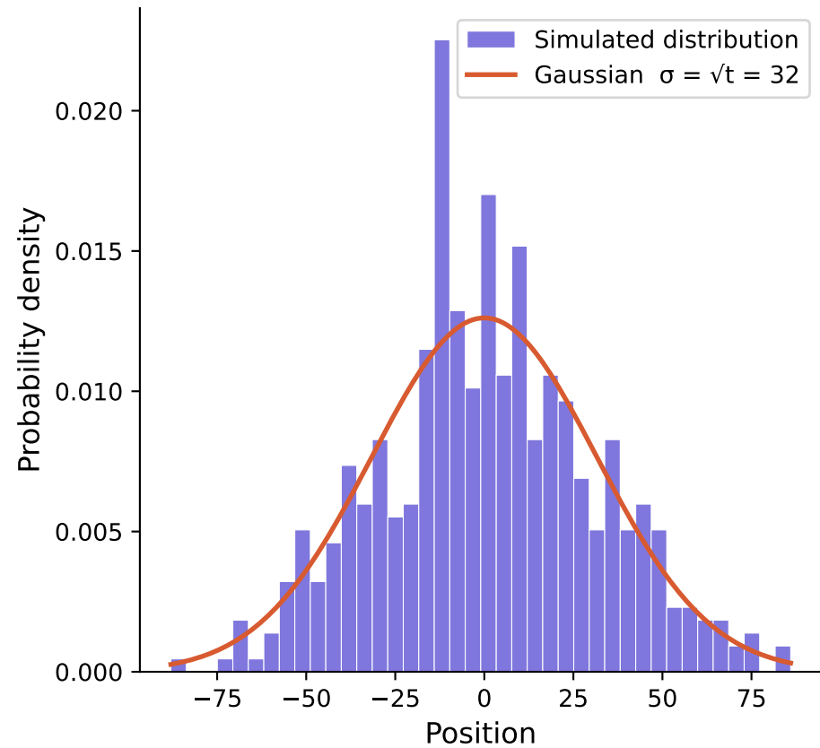
Position distribution at t = 1000
