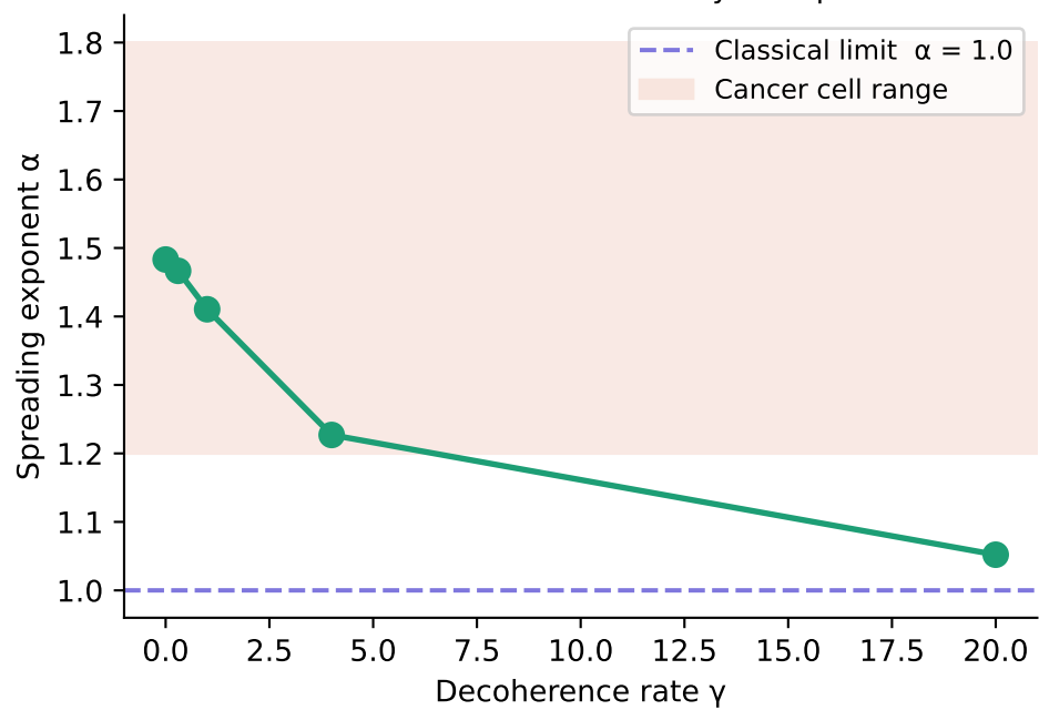
\alpha decreases monotonically with \gamma
