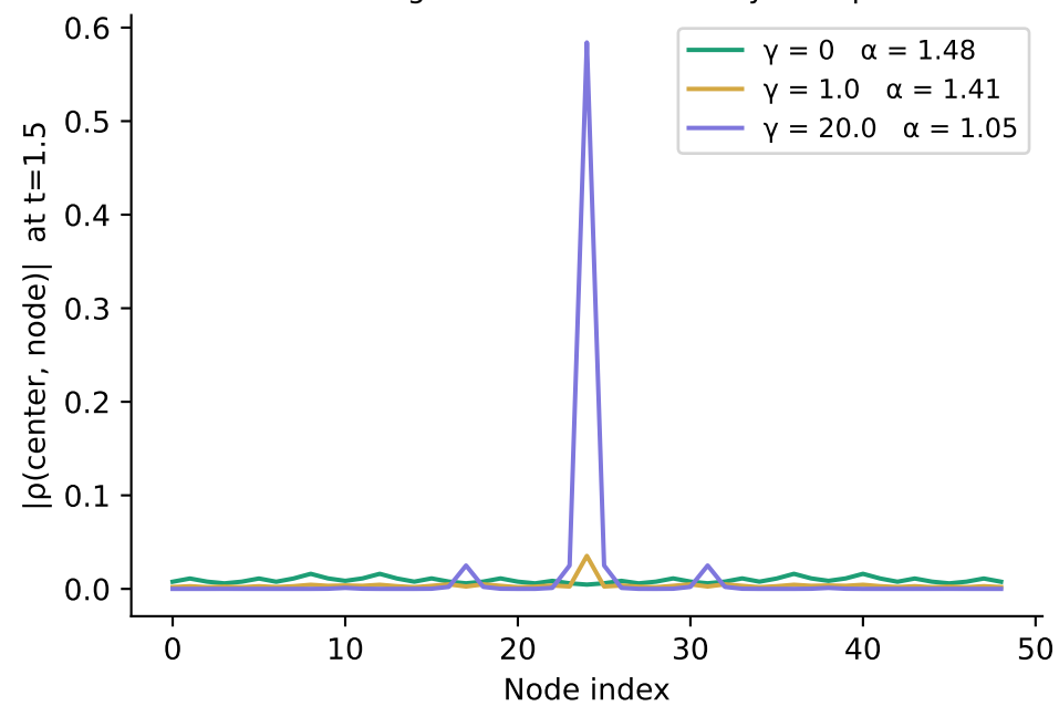
Off-diagonal coherences decay with \gamma
