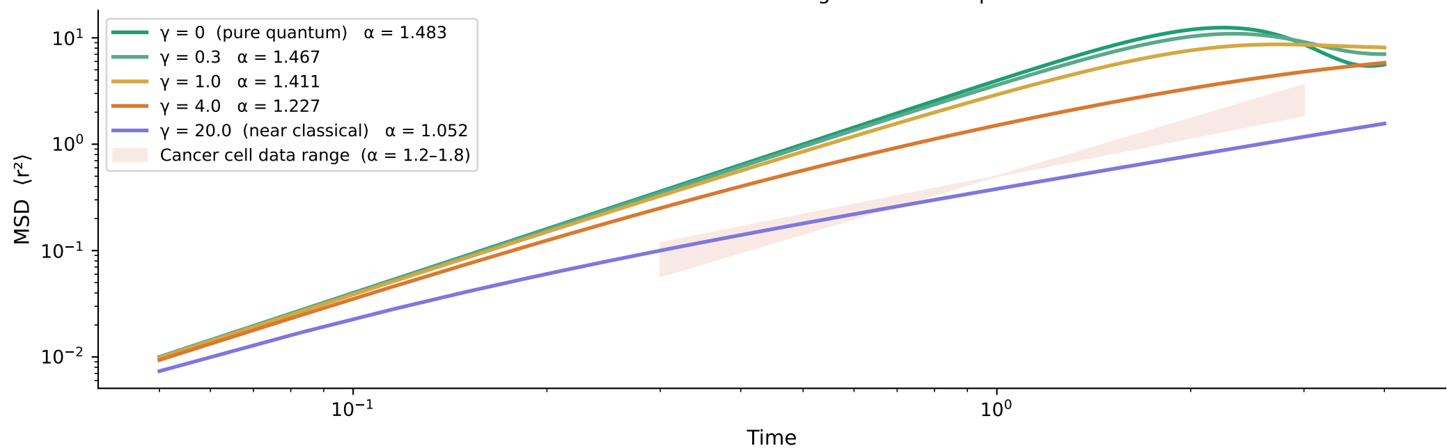
MSD vs time for increasing decoherence \gamma
