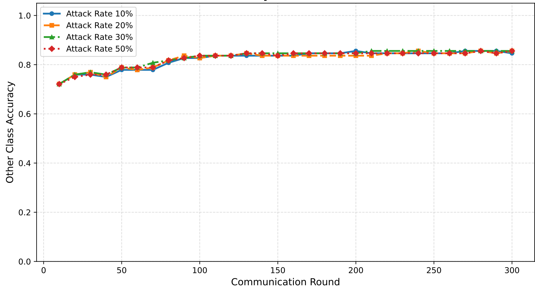
Other Class Accuracy vs Communication Round
