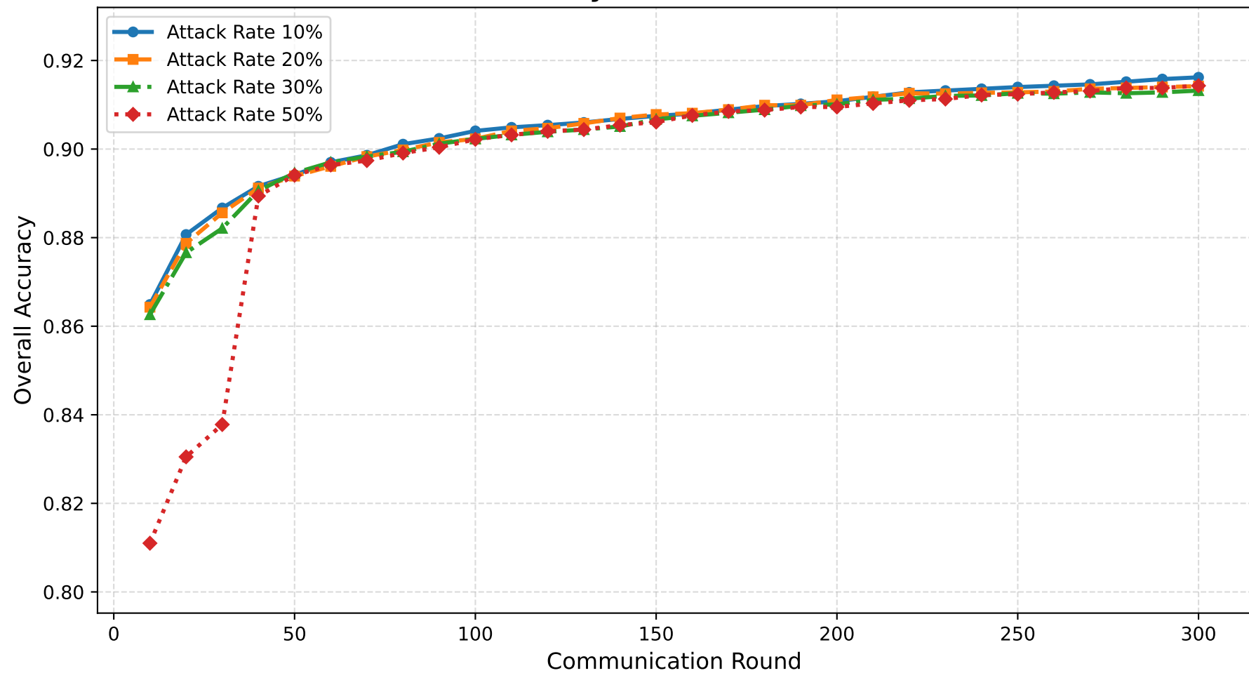
Overall Accuracy vs Communication Round
