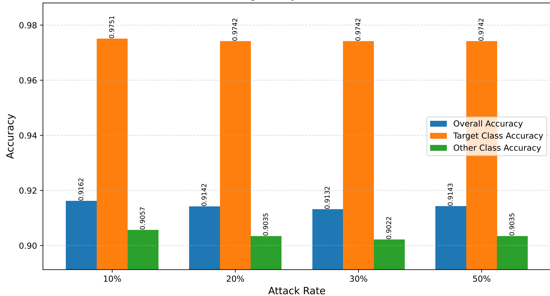
Final Accuracy Comparison at Round 300
