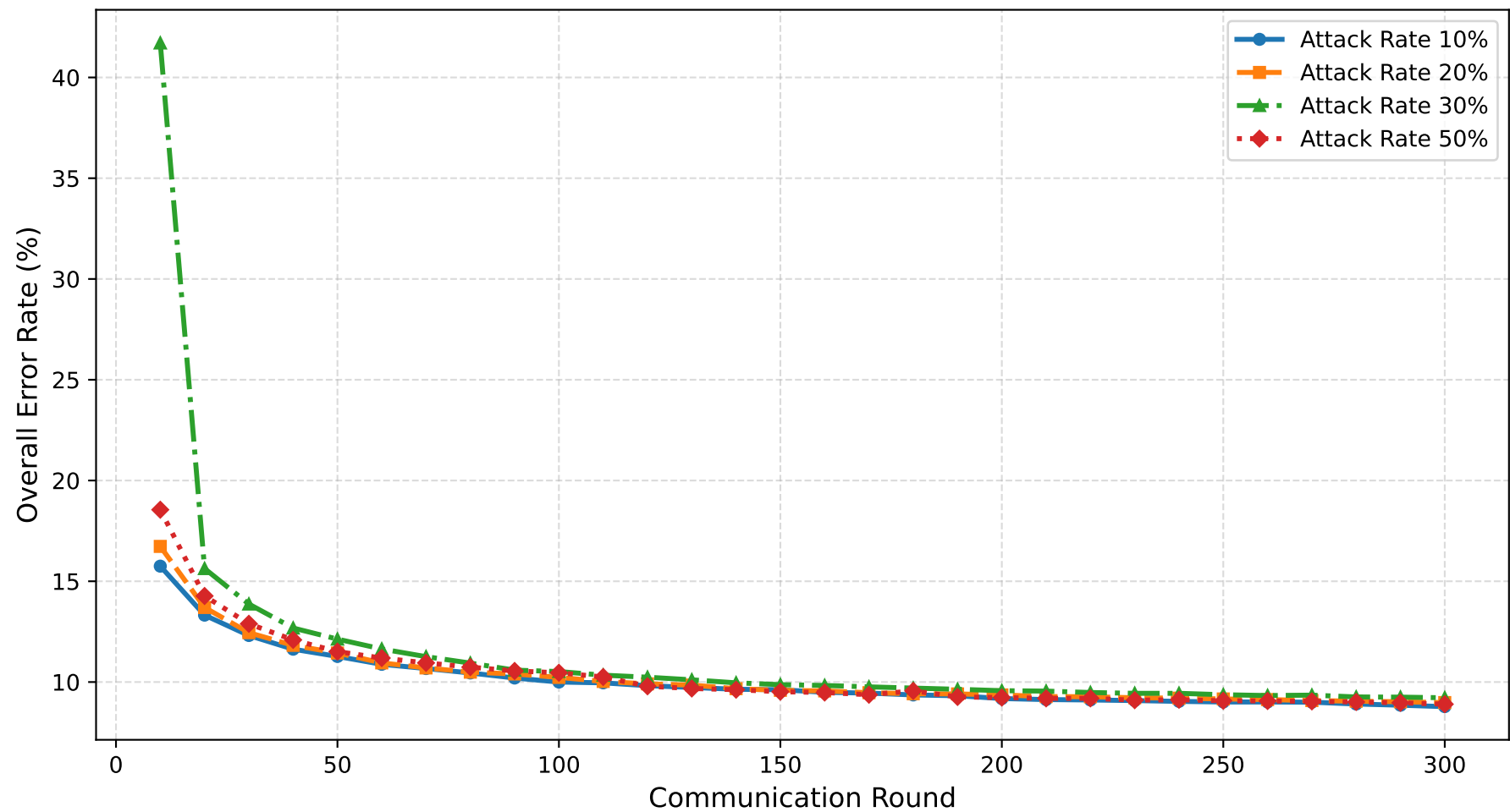
Overall Error Rate vs Communication Round
