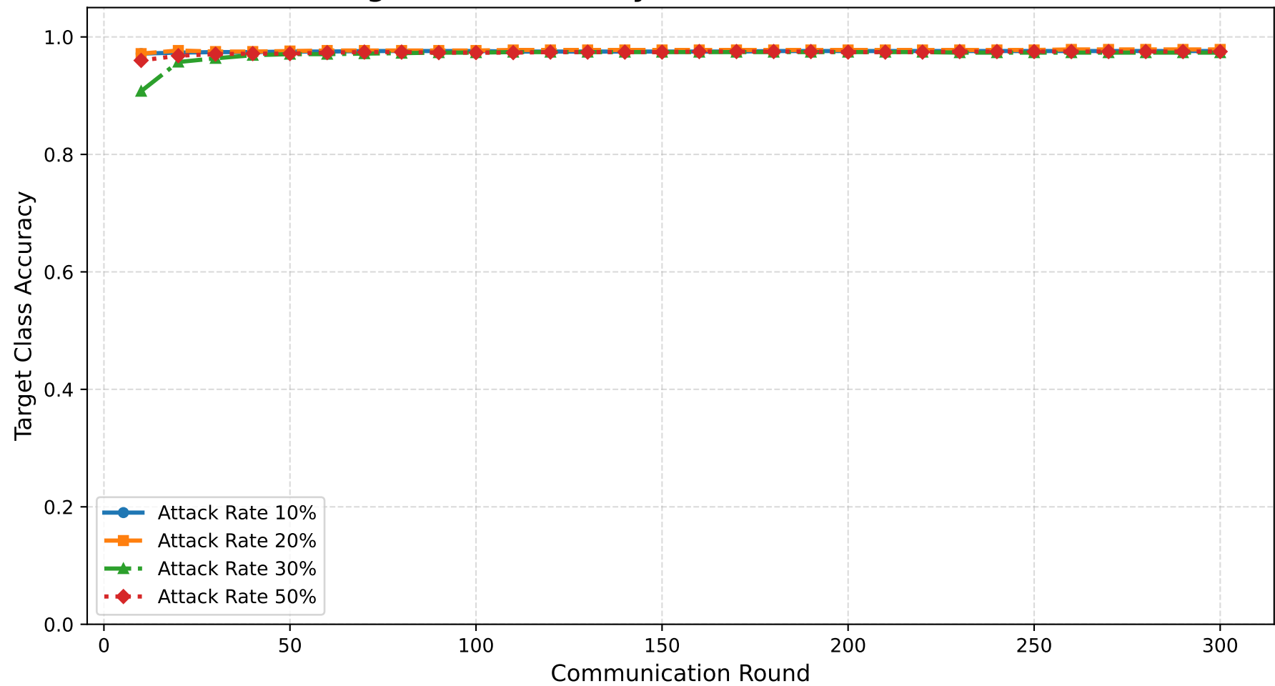
Target Class Accuracy vs Communication Round
