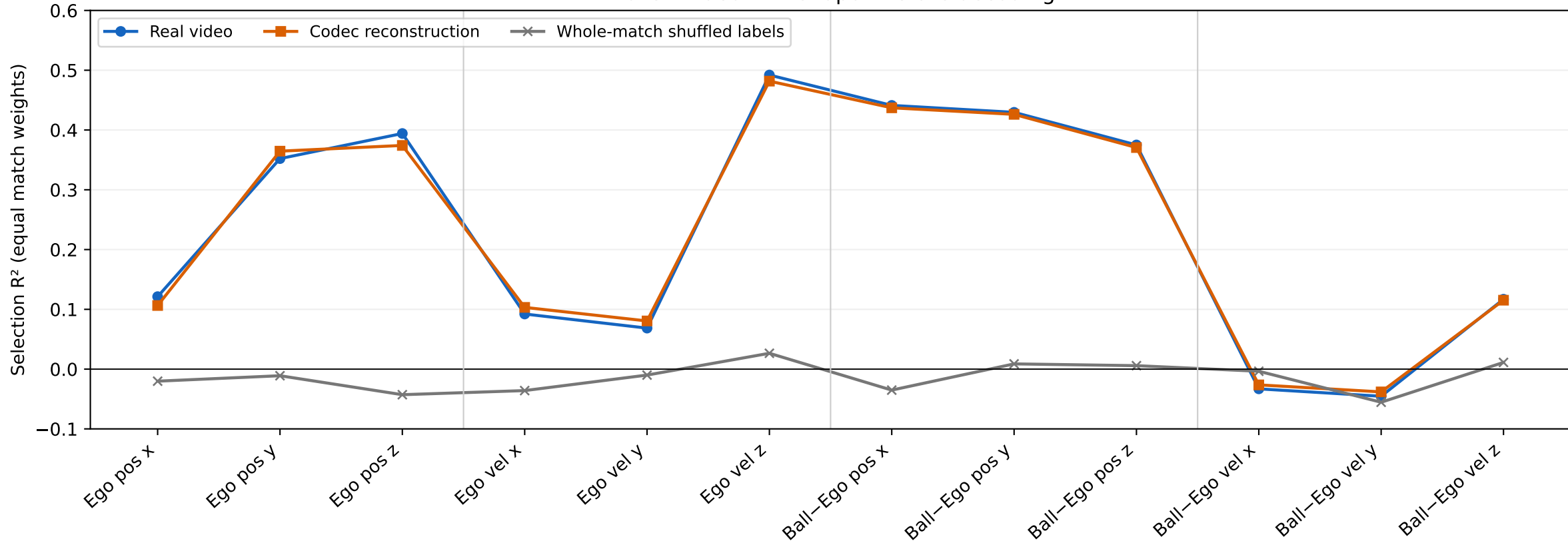
Frozen VideoMAE endpoint state decoding
