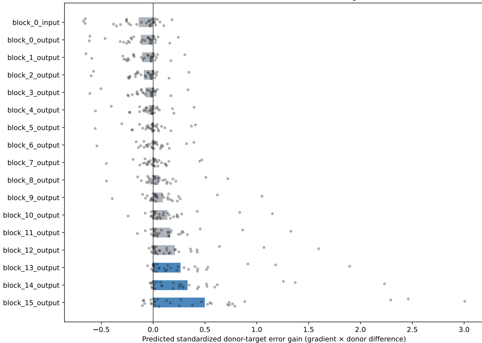
All 17 discovery sites; blue marks the frozen top 3 Bar: mean across 31 matches; dots: each match averaged over 2 seeds
