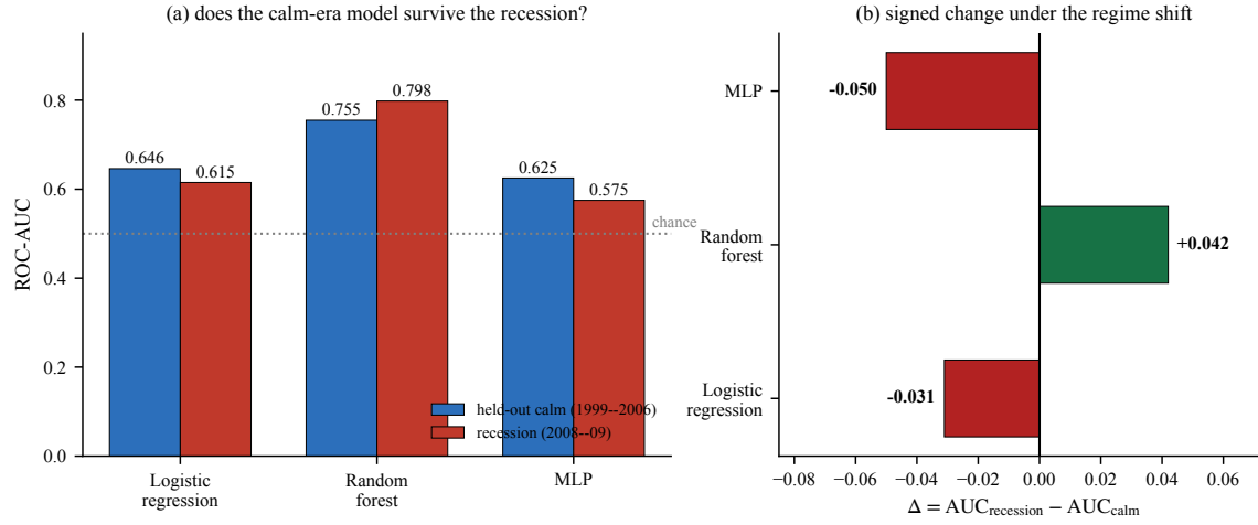
Fig. 3. (a) Calm versus recession ROC-AUC per model. Taller red than blue means the model holds up. (b) The signed change of Eq. (5): only the random forest is positive, and it is the only model that was strong to begin with.
