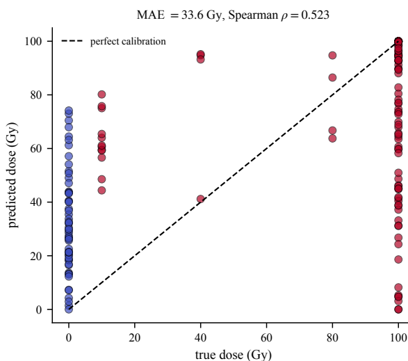
Fig. 6. Secondary task: exact-dose regression under the same leave-one-study-out protocol. Predictions cluster in the interior, the signature of a model separating two groups rather than estimating a continuous quantity.
