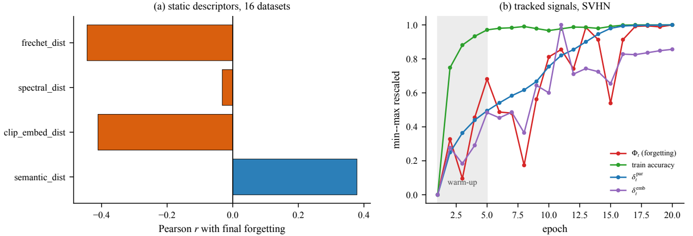
Fig. 3. (a) Pearson correlation of each static descriptor with final forgetting across the 16 datasets. All are modest and estimated from 16 points. (b) The four tracked signals for SVHN at \eta = 10^{-5} , min-max rescaled; the shaded region is the K = 5 warm-up.
