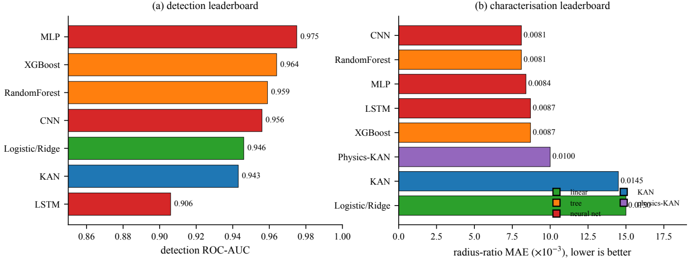
Fig. 2. (a) Detection ROC-AUC and (b) characterisation MAE in R_p/R_* , coloured by model family. Note the axis scales: the detection spread is 0.069 AUC across all seven families, whereas the characterisation spread is nearly a factor of two in error.
