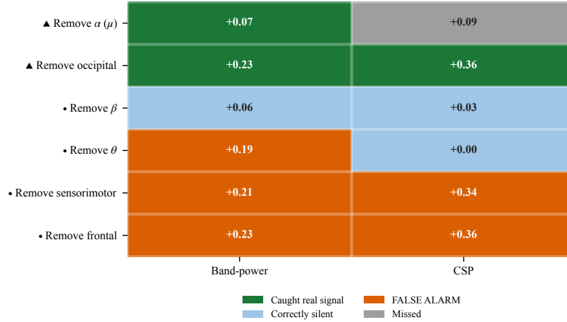
Figure 5: Real-brain validation on eyes-open versus eyes-closed, 34 PhysioNet subjects, where physiology fixes the truth to occipital alpha. Triangles mark controls that should fire, dots those that should stay silent; cells give the accuracy drop. Band-power false-alarms on three of four absent targets, CSP on both spatial ones.
