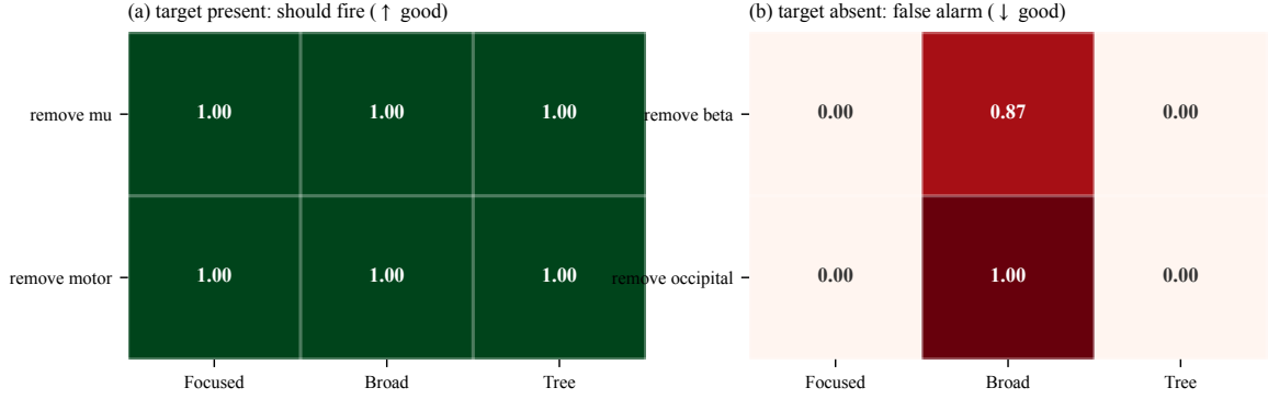
Figure 2: Measured fire rates over 15 simulated datasets. (a) All three decoders detect the genuinely planted dependence. (b) The linear BROAD decoder false-alarms on 87% of \beta removals and 100% of occipital removals, where no signal exists. TREE sees the identical 38 features and never false-alarms.
