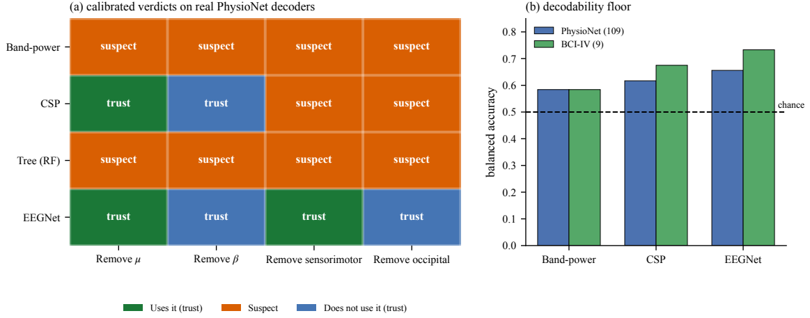
Figure 4: (a) Calibrated verdicts on real PhysioNet decoders. Each cell attaches the measured reliability of Figure 3 to the observed accuracy drop, converting “the control fired” into a trust-weighted statement. Band-power and the tree earn no trustworthy verdict on any control; EEGNet earns four. (b) Held-out balanced accuracy: all decoders read motor imagery above chance.
