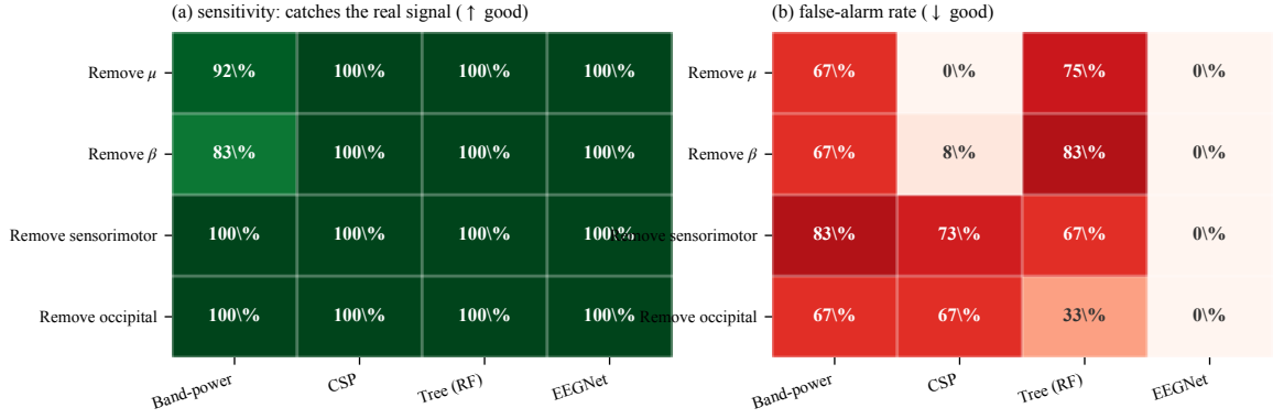
Figure 3: Measured operating characteristics on the simulator grid. (a) Sensitivity is high everywhere: all four decoder families detect genuine dependence. (b) False-alarm rates differ by more than an order of magnitude. Band-power fires on 67–83% of perturbations whose targets are absent; EEGNet essentially never does.
