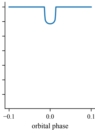
small planet R_p/R_* = 0.05
