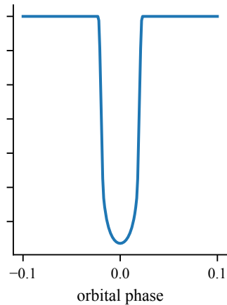
tighter orbit a/R_* = 8
