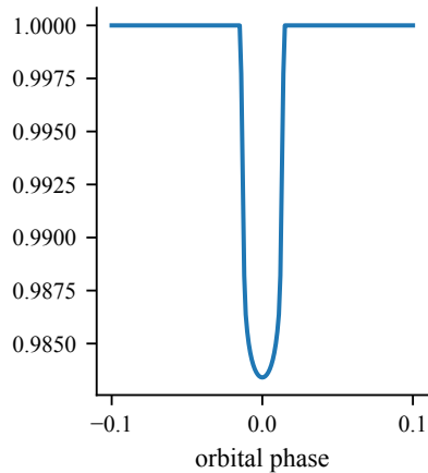
large planet R_p/R_* = 0.12
