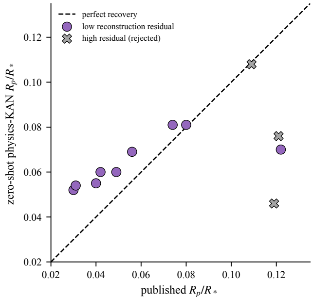
(b) full-sample MAE = 0.023; screened-subset MAE = 0.018
