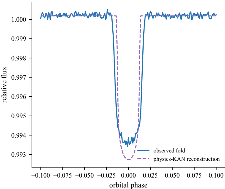
(a) a real Kepler fold: Kepler-719 b
