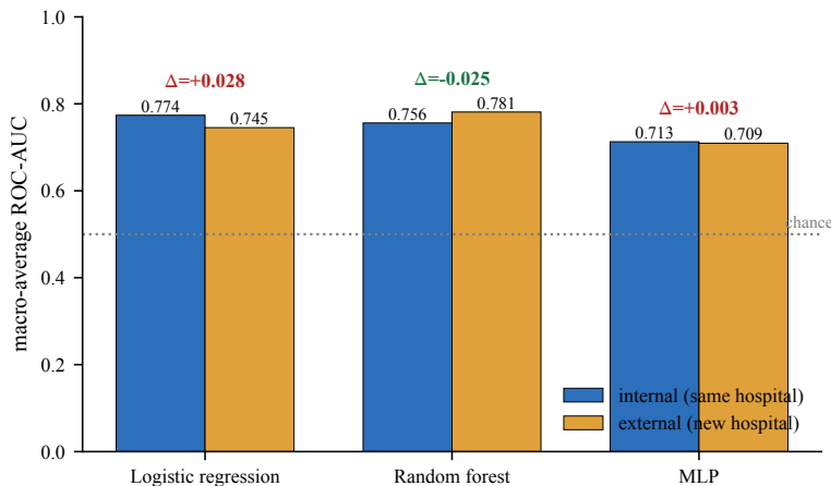
Figure 4: Macro-averaged internal versus external discrimination. The MLP has the smallest magnitude gap and the worst absolute performance; the random forest has a negative gap and the best absolute external performance. Ranking models by |\Delta| would select the weakest model.
