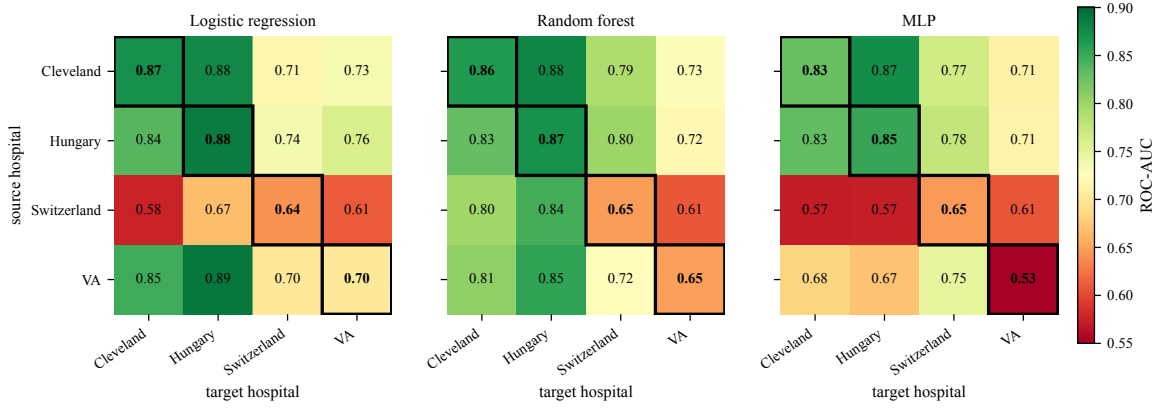
Figure 2: Directed transfer matrices of ROC-AUC on the nine portable variables ( \mathcal{F}_9 ). Rows index the source hospital used for fitting, columns the target hospital used for scoring. Boxed diagonal cells are within-site five-fold cross-validation with preprocessing refitted per fold; all other cells are strict source-only fits scored on an untouched target. The dominant structure is horizontal (source-driven), not vertical.
