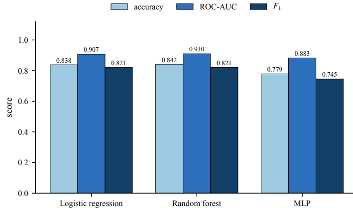
Figure 1: Internal Cleveland performance under stratified five-fold cross-validation with all thirteen predictors. The two classical learners are separated by less than one standard error of the AUC at this sample size; the neural network is not competitive.
