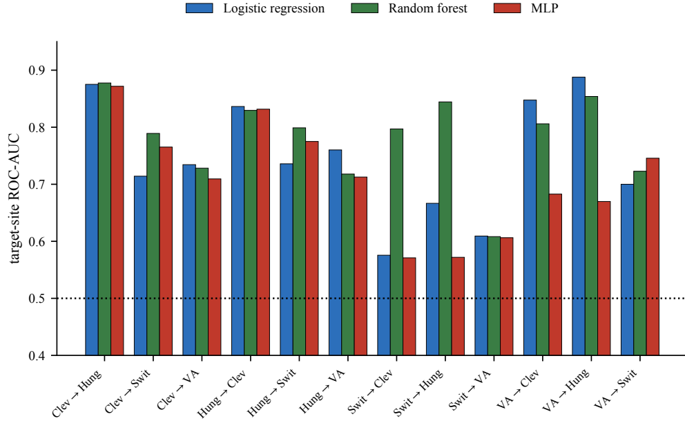
Figure 3: The twelve directed transfers, grouped by source→target pair. The spread within a pair (model choice) is generally smaller than the spread across pairs (cohort choice), except where the source cohort is degenerate (Switzerland), in which case model choice becomes decisive.
