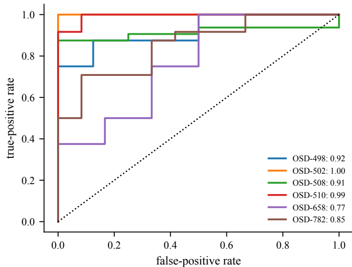
(b) ROC per completely held-out study
