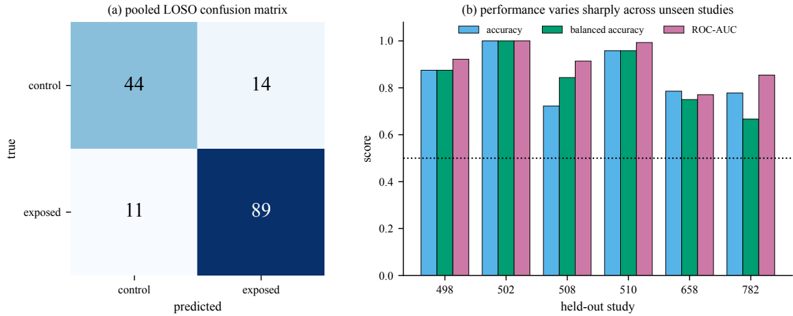
Figure 3: (a) Pooled confusion matrix for the stability ensemble. Specificity (75.9%) lags sensitivity (89.0%). (b) Per-study performance. OSD-502 is perfectly classified and OSD-510 nearly so, while OSD-782 falls to 66.7% balanced accuracy despite an AUC of 0.854—a threshold problem, not a ranking failure.
