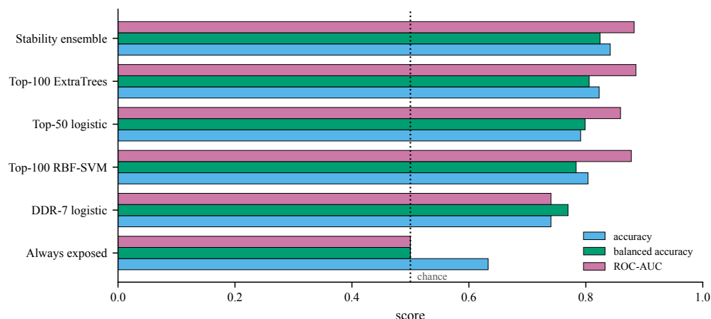
Figure 2: The model ladder. The always-exposed rule attains 0.633 accuracy with 0.500 balanced accuracy and zero specificity, which is exactly why accuracy is not the primary endpoint. Fold-local multigene models improve substantially on the literature panel.
