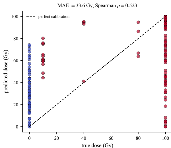
Figure 6: Secondary task: exact-dose regression under the same leave-one-study-out protocol. Predictions cluster in the interior, the signature of a model separating two groups rather than estimating a continuous quantity.
