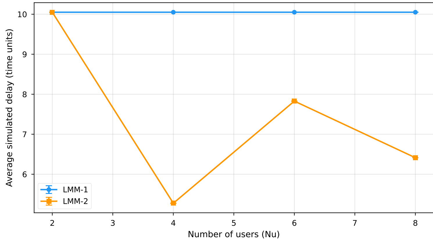
LMM-1 vs LMM-2: Routing Delay vs User Count ( N_p=10 ) (with chunking, with auth)
