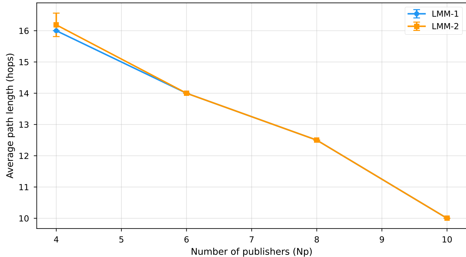
LMM-1 vs LMM-2: Path Length vs Publisher Count (with chunking, with auth)
