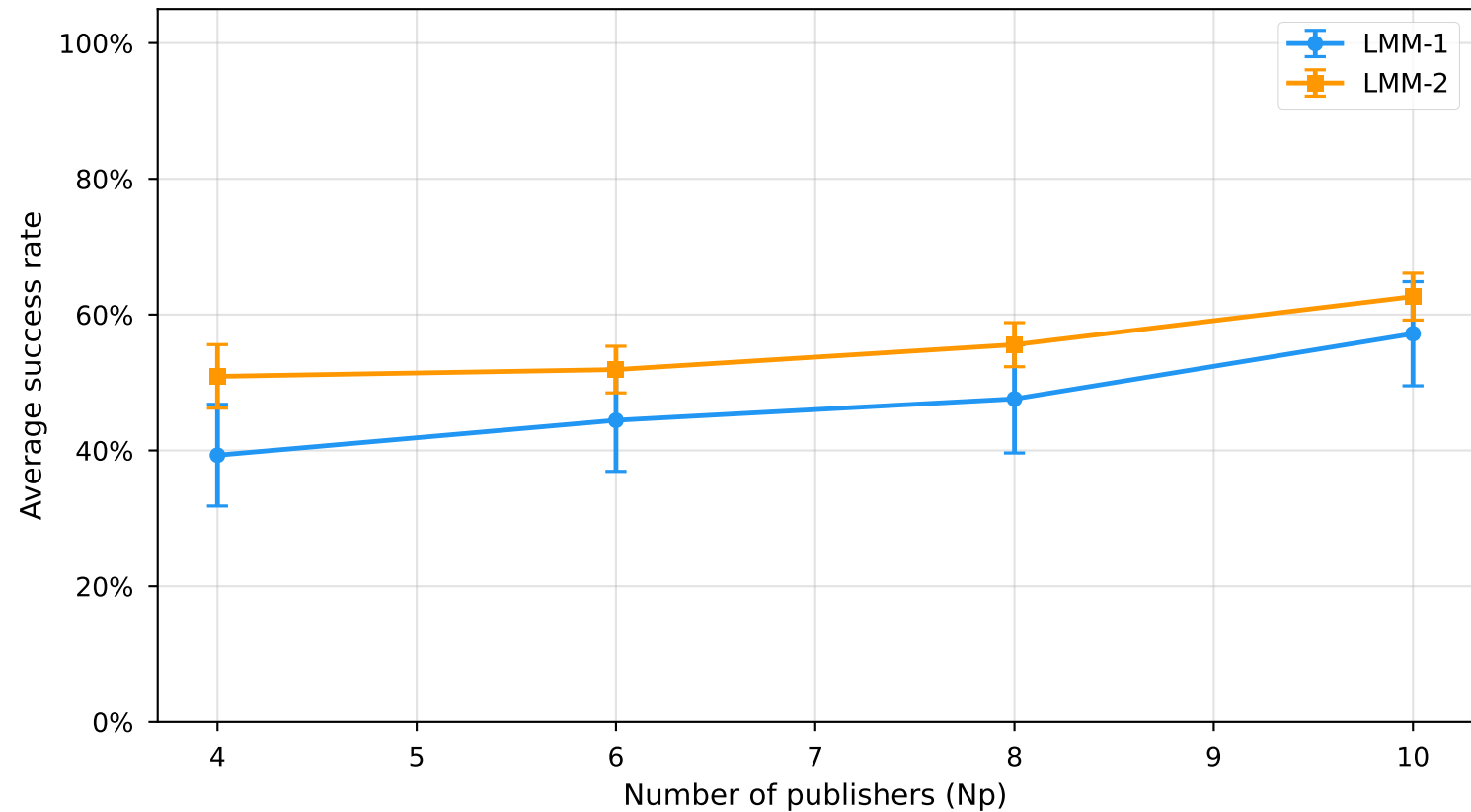
LMM-1 vs LMM-2: Success Rate vs Publisher Count (with chunking, with auth)
