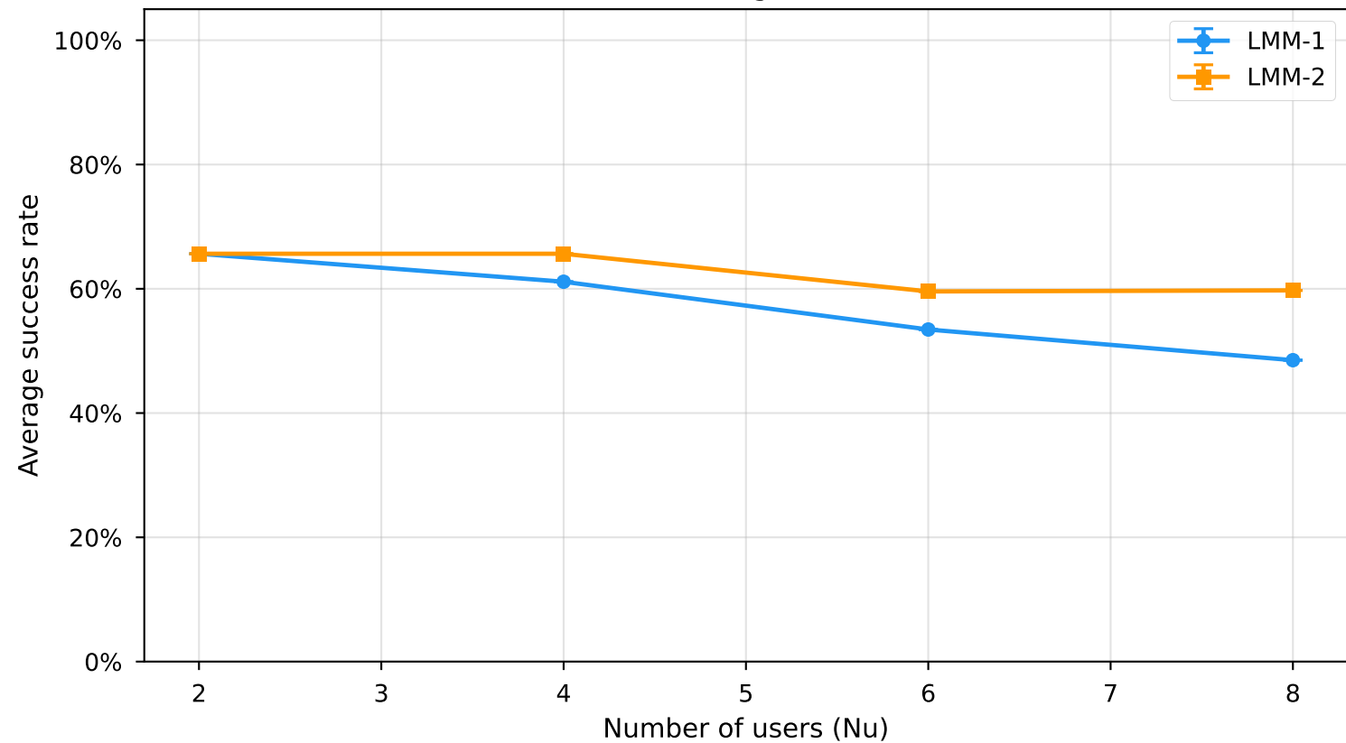
LMM-1 vs LMM-2: Success Rate vs User Count ( N_p=10 ) (with chunking, with auth)
