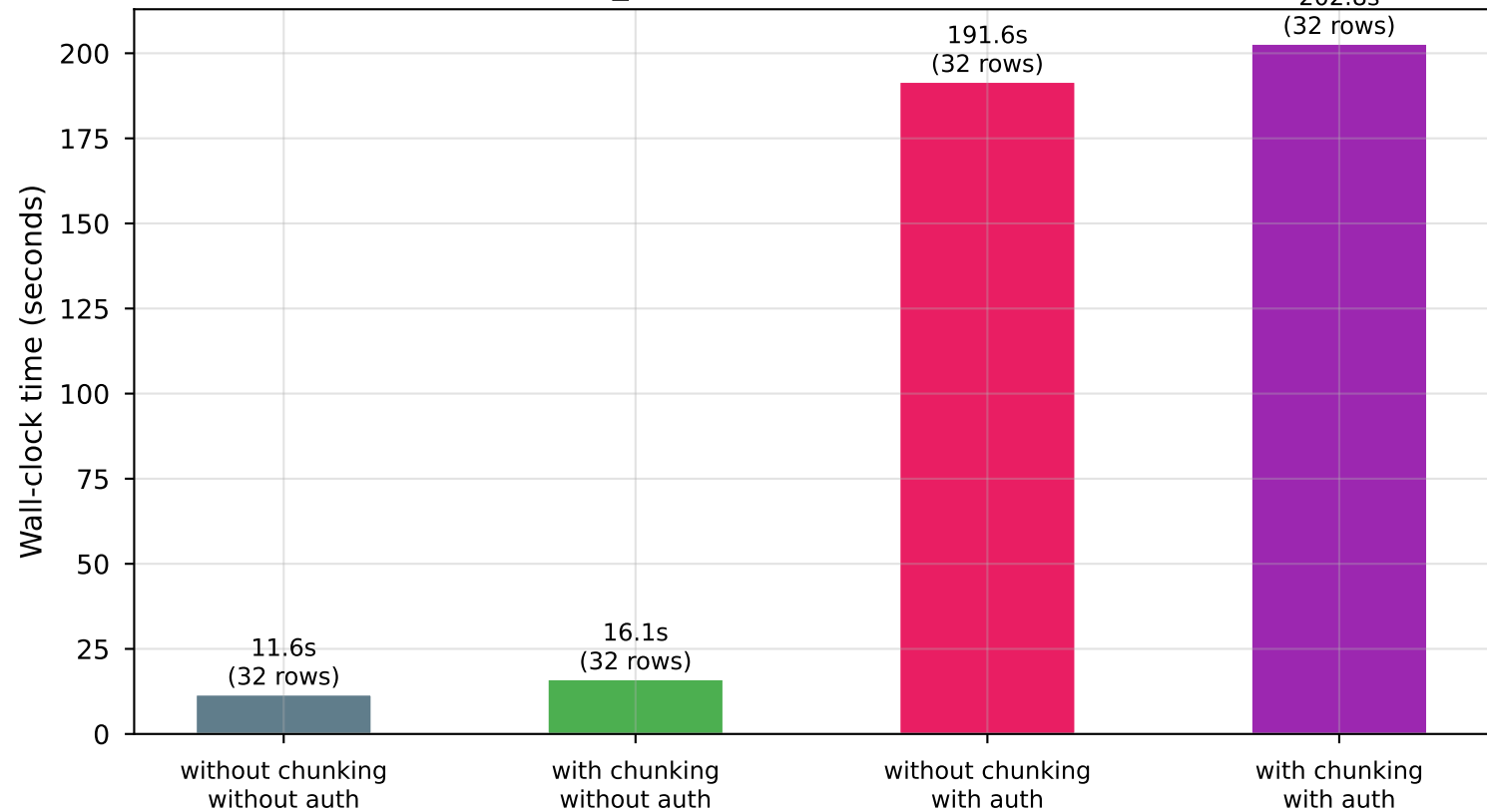
Authentication Overhead: Total Benchmark Duration per Mode (1 iterations; with_auth runs include Fabric gRPC roundtrips)
