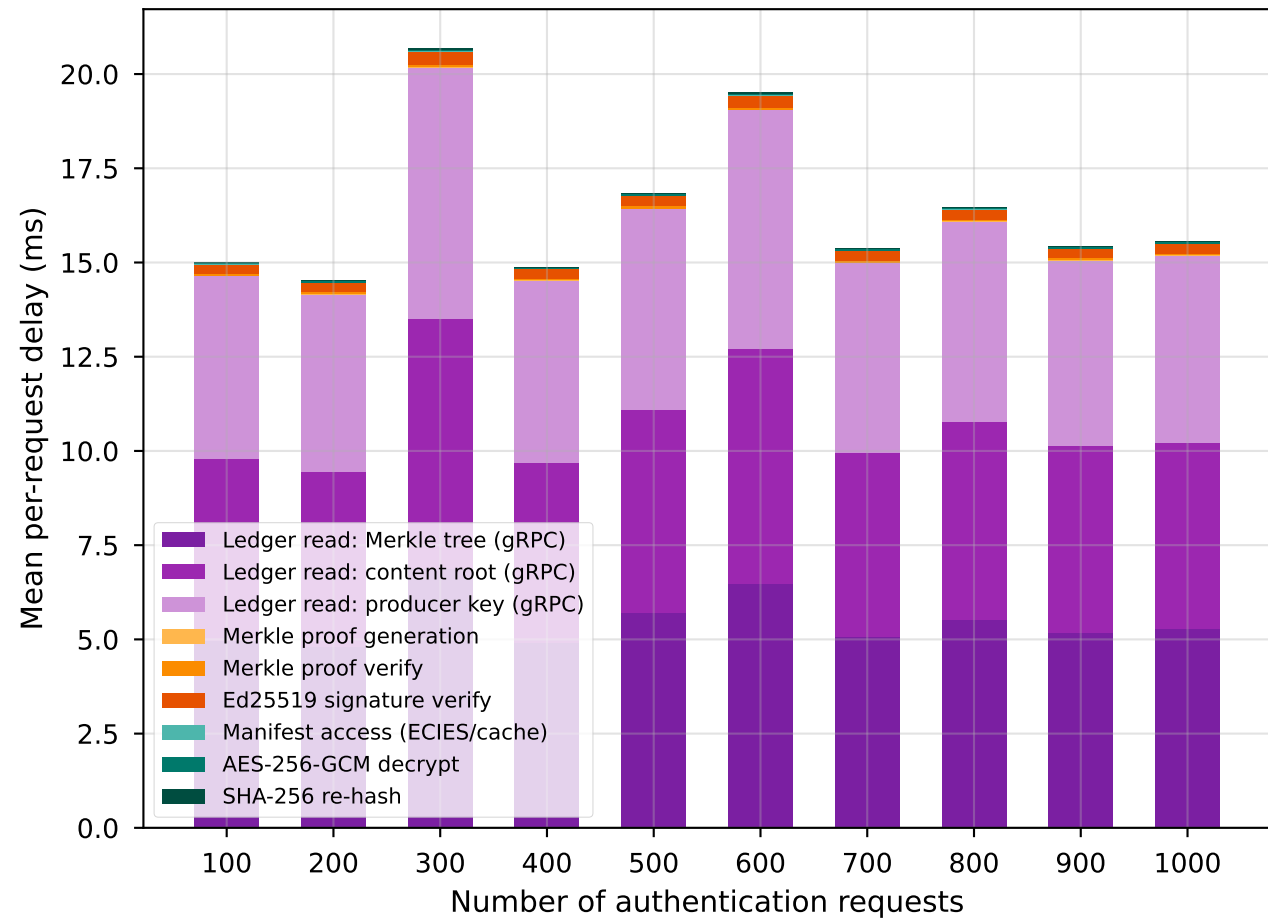
(b) Decomposition of per-request authentication delay (proposed, Fabric ledger)
