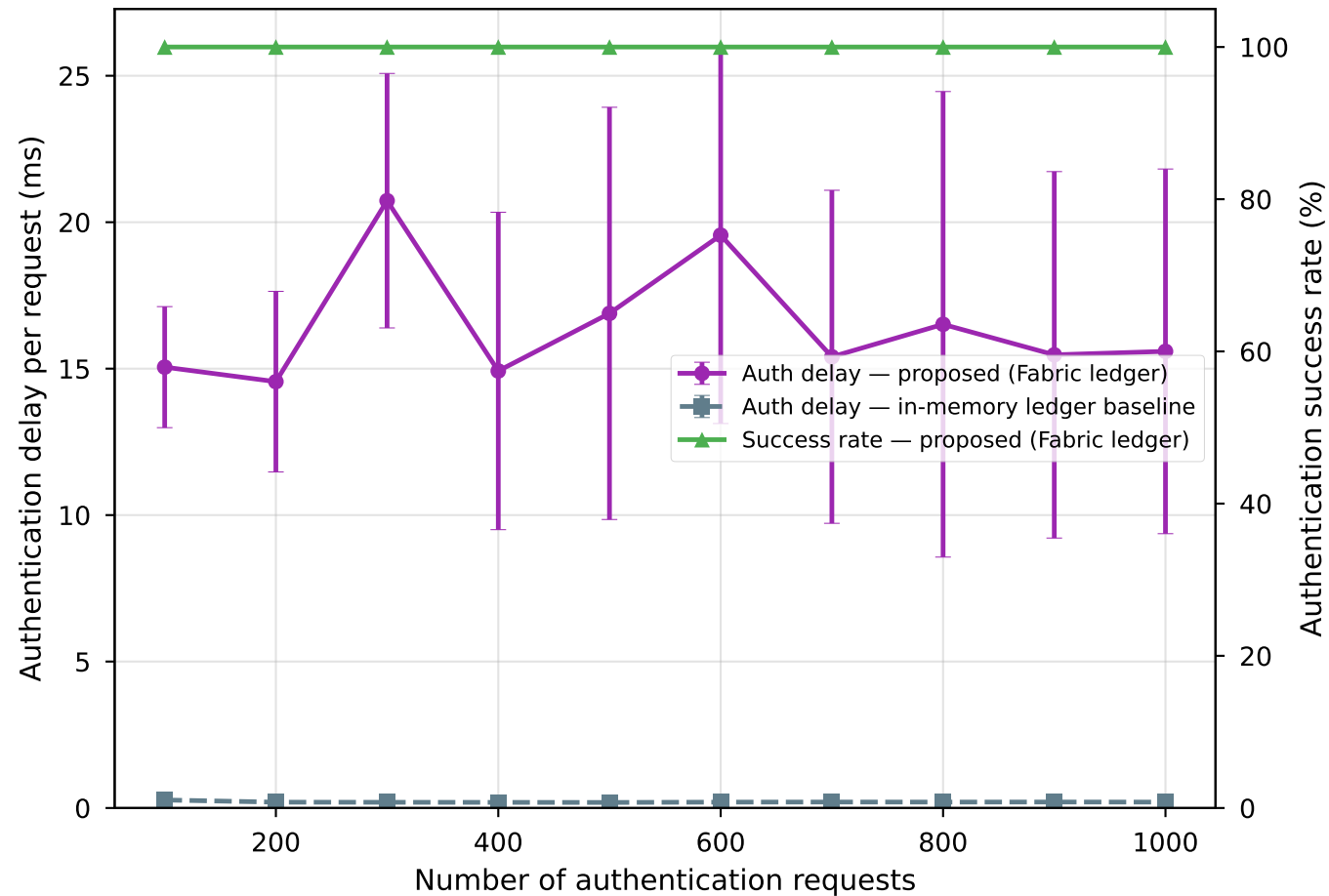
(a) Authentication delay and success rate vs. number of requests
