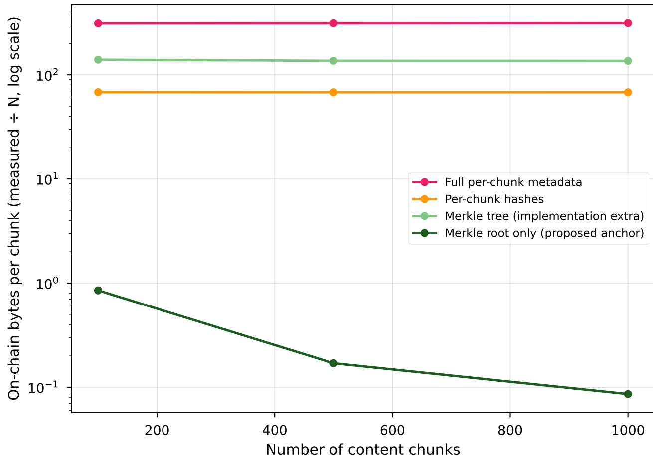
(b) Amortised on-chain cost per chunk (derived: measured bytes \div chunk count)
