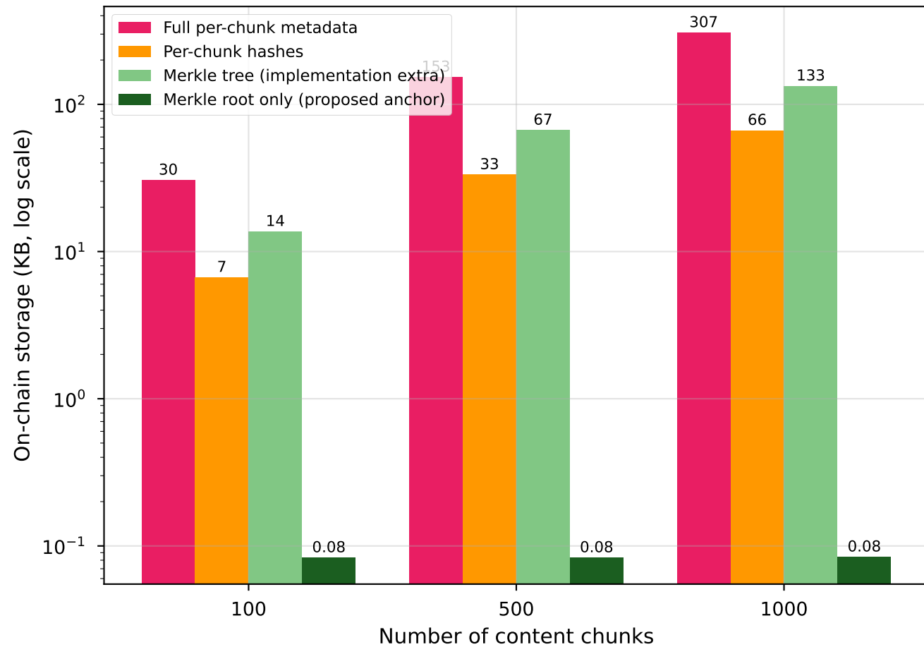
(a) Measured on-chain storage per content object by storage strategy
