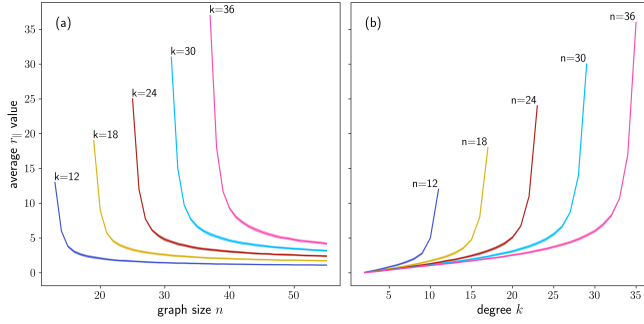
Fig. 2: Variation in bounds of validity for Lyapunov–Schmidt reduction for consensus bifurcation over balanced regular graphs. For each (n, k) pair, 100 independent random graphs were generated using the NetworkX package in Python. The reported mean values and corresponding error bars represent the average and standard deviation of the computed bounds on r_{\parallel} across the sampled graphs. (a) illustrates the bounds with fixed degree k \in \{12, 18, 24, 30, 36\} , varying graph size n ; (b) illustrates the bounds with fixed graph size n \in \{12, 18, 24, 30, 36\} , varying degree k .
