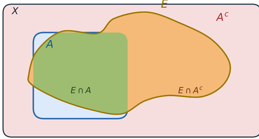
Figure 1: Within X , blue represents A , red represents A^c , and yellow represents E . Their overlap is green in E \cap A and orange in E \cap A^c .
