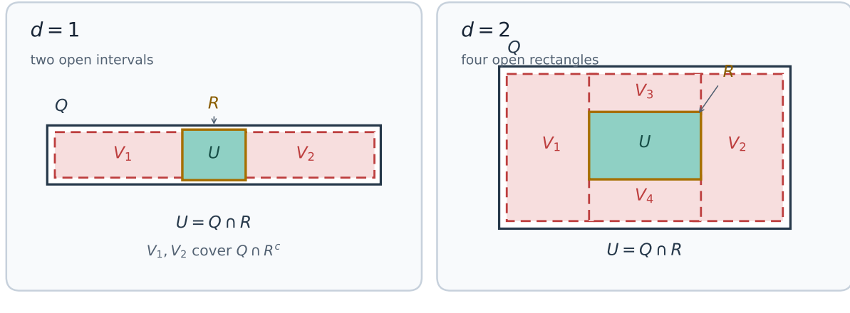
Figure 3: The part of an open rectangle Q outside an open rectangle R can be covered by at most 3^d open rectangles V_r , while U = Q \cap R is itself open. Dashed boundaries indicate the arbitrarily small enlargement used to keep every covering rectangle open.
