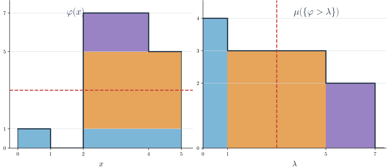
Figure 1: The graph of \varphi (left) and the function \lambda \mapsto \mu(\{x \in E : \varphi(x) > \lambda\}) (right). Matching colors represent equal areas in the two panels.
