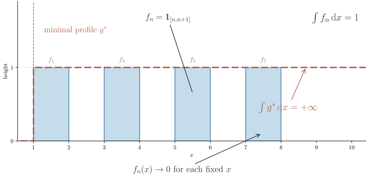
Figure 2: The unit-mass wave moves to the right and converge pointwise to zero. The minimal dominating profile is non-integrable: \mathbf{1}_{[1, \infty)} .
