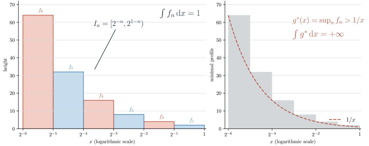
Figure 3: The unit mass is packed into intervals shrinking toward zero. The minimal dominating profile has the same non-integrable singularity as 1/x .
