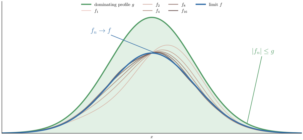
Figure 1: A sequence of functions f_n that converge to a limit function while remaining below one fixed dominating profile g .
