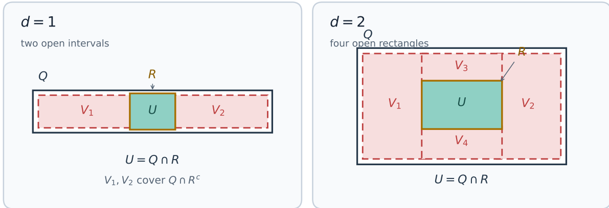
Figure 3: The part of an open rectangle Q outside an open rectangle R can be covered by at most 3^d open rectangles V_r , while U = Q \cap R is itself open. Dashed boundaries indicate the arbitrarily small enlargement used to keep every covering rectangle open.
